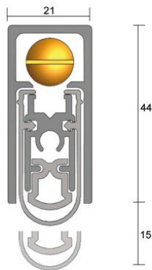
Threshold automatic drop seal: IS8520si
