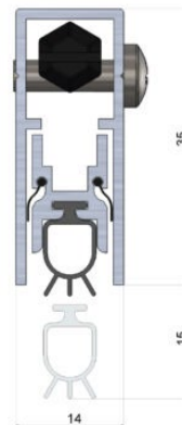
Drop seal: IS8011si
