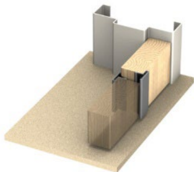
Dual leaf door meeting stile: IS7061si x 2
