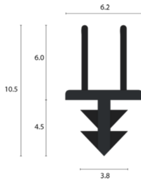
Perimeter seal: IS0511
